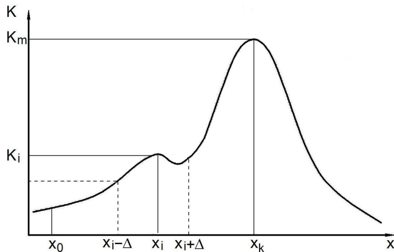
Abbildung 2.7: Metropolis-Hastings Sampling.
