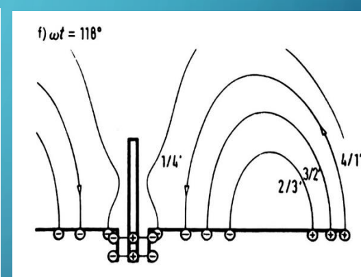
Fig. 7(f): Radiation patterns as a function of different \omega t ( \omega t = 118^\circ )
