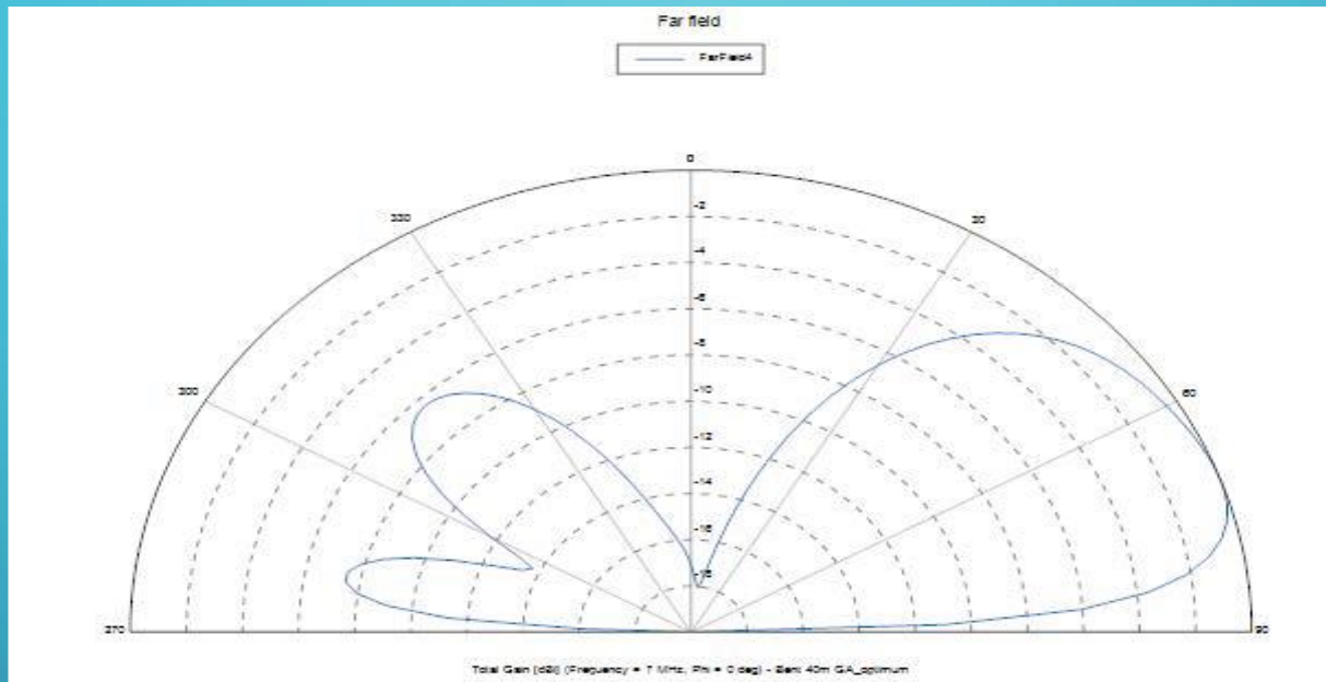
Figure 24: Elevation Pattern
