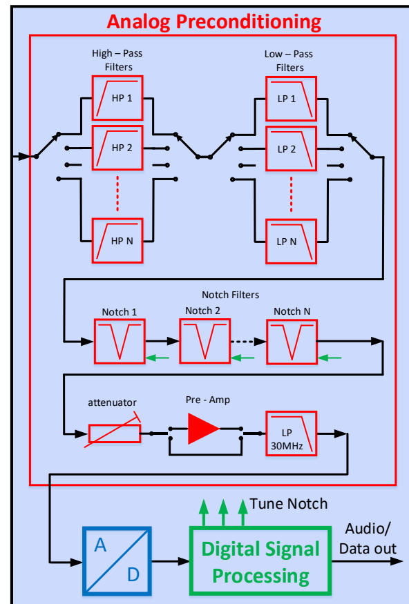
Δ Fig. 7 Wideband HF receiver
