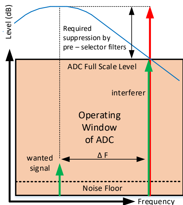
Δ Fig. 8 ADC Operating Window with Pre - Selector
