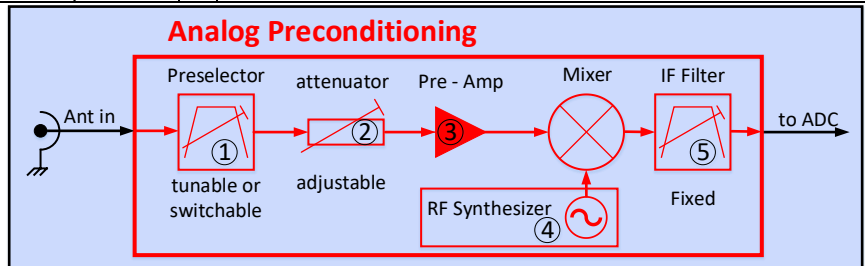
Δ Fig. 3 Analogue preconditioning for IF sampling
