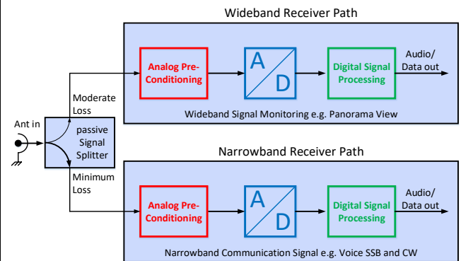
Δ Fig. 5 SDR Receiver Structure
