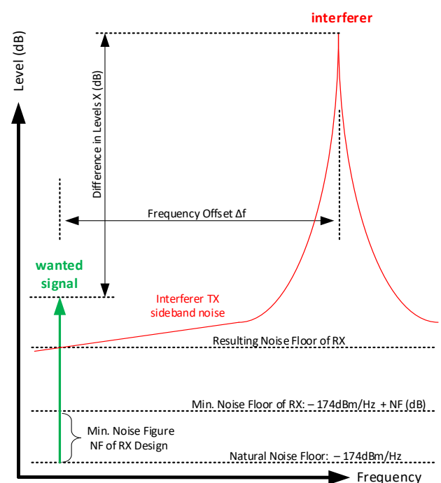
Δ Fig. 10 Key Parameters for collocated Installations
