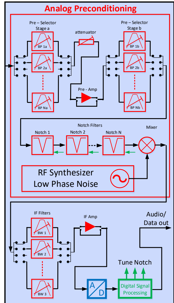
Δ Fig. 11 High End SDR Receiver Block Diagram
