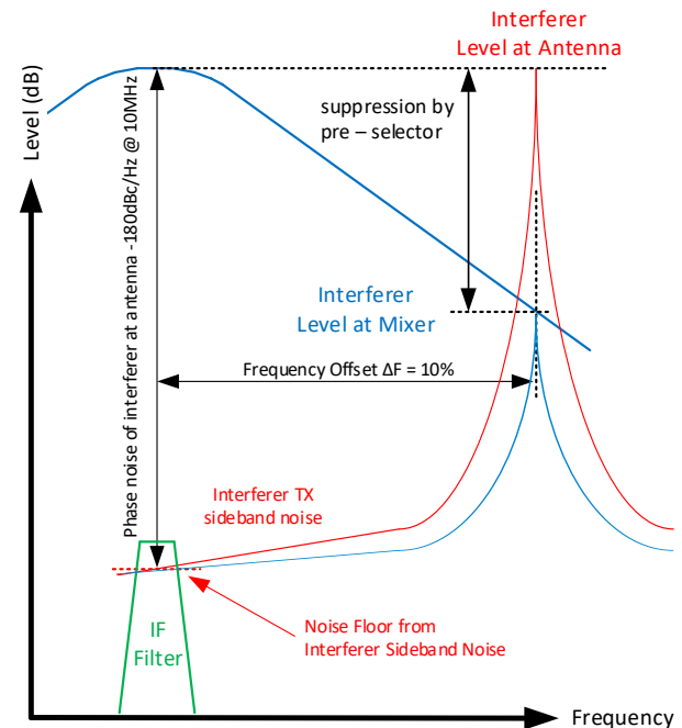
Δ Fig. 12 Phase Noise at Mixer
