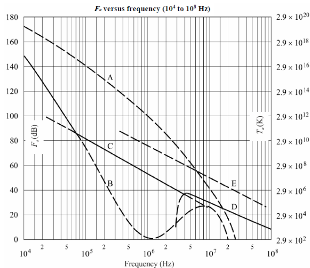
Δ Fig. 6 Noise external to an HF receiver
