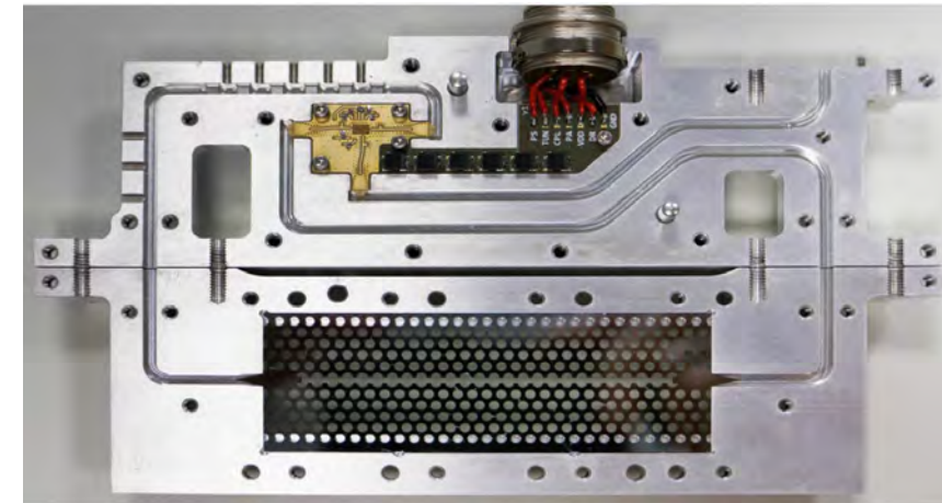
Fig. 3 MMIC VCO assembly in its housing (top half removed) [Ref.,].
