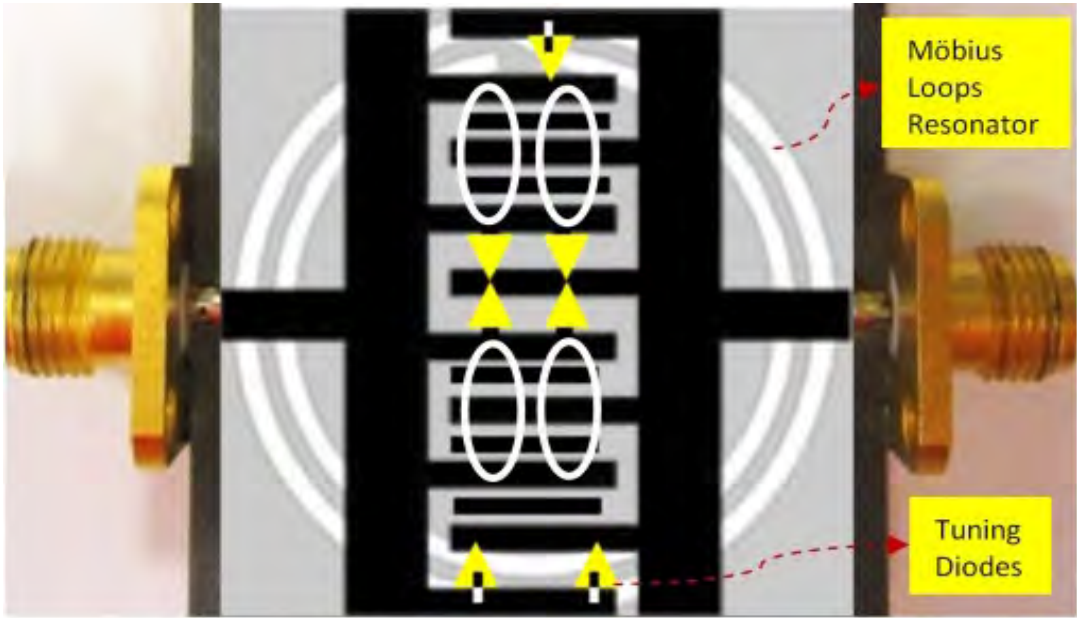
Printed Möbius Metamaterial Resonator
