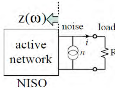
Equivalent noise model of NISO
