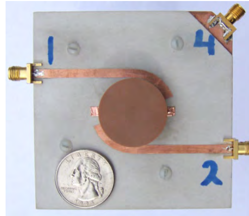
Dual Band Dielectric Resonator Antenna & Filter
