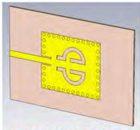
Complimentary CR
