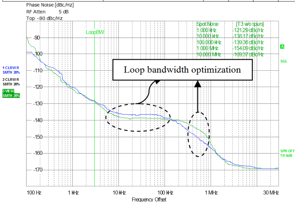
A typical measured phase noise plot of the 10.24 GHz synthesized signal source
