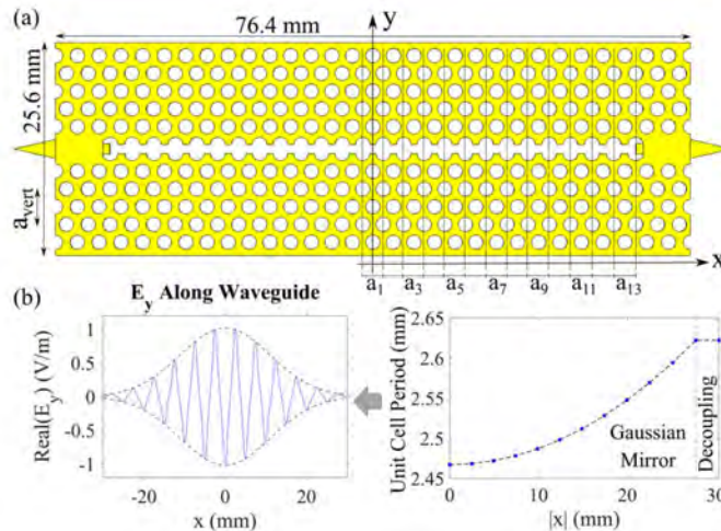
Fig. 2. (a) EBG resonator with its dimensions and variable periodicity ( a_n ) along the x-axis. (b) Gaussian envelope of the resonant mode achieved by linearly increasing the reflection from the center to the outer unit cells [Ref.1]
