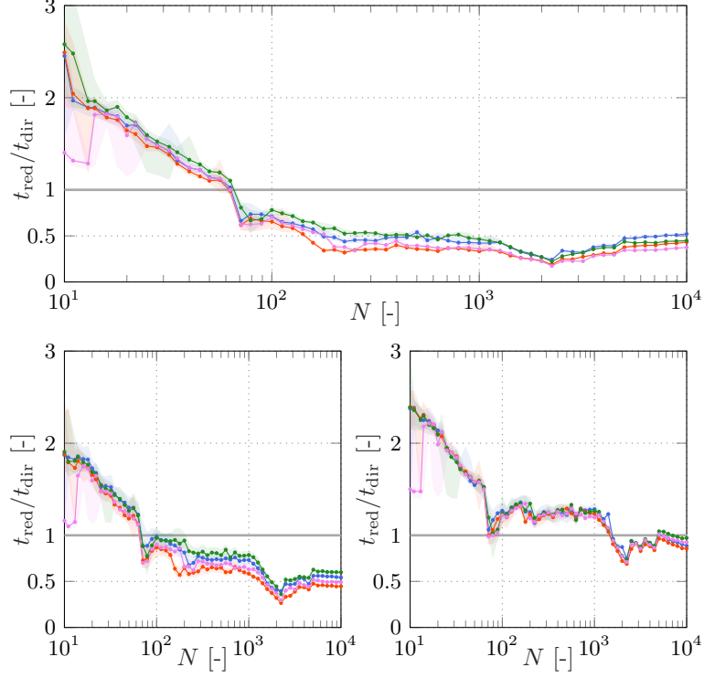
Figure 4: Ratio of execution time: \mathcal{I}_{\text{re}}^t (top), \mathcal{I}_{\text{re}}^{\text{ts}} (bottom left), \mathcal{I}_{\text{re}}^s (bottom right); full matrices. Median value (line) and 9%-91% quantiles (filled area).
