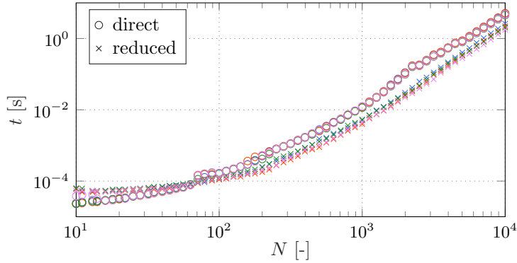
Figure 3: Execution time: direct approach ( t_{\text{dir}} , dot) and reduced approach ( t_{\text{red}} , cross) with reduction set \mathcal{I}_{\text{re}}^t ; full matrices. Median value.
